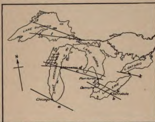
FIG. 374. — Map of the Great Lakes region to show isobases and hinge lines of uptilt. a , isobase of the Chicago outlet; b , main hinge line of the Lake Whittlesey beach (Leverett); b 1 , hinge line of the Lake Warren beach (Taylor); c , isobase of the Port Huron outlet; d , main hinge line of highest Algonquin beach (Goldthwait); e , f , g , h , additional hinge lines of Algonquin beaches in Door County peninsula (Hobbs); l , isobase of the Lake Superior outlet for the Algonquin beaches (Leverett); m , isobase of the same outlet for the Nipissing beaches (Leverett).
